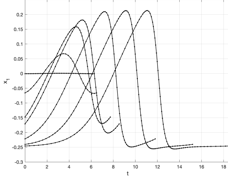
Figure 18: Time histories for labeled periodic orbits found during continuation using the code in Sect. 7.4.
