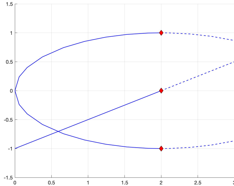
Figure 11: Bifurcation diagram showing real and imaginary parts of the eigenvalues of the Jacobian of the vector field with respect to the state versus the parameter B for the vector field in Section 3.4. The red diamonds mark the Hopf bifurcation.
