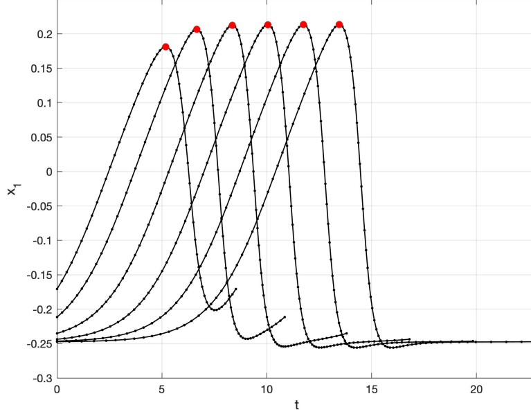
Figure 20: Time histories for labeled periodic orbits found during continuation using the code in Sect. 7.4 with a family of local maxima highlighted using red disks.
