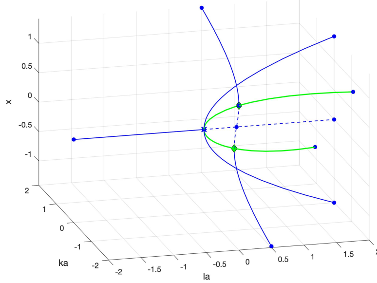
Figure 3: Bifurcation diagram showing branches of asymptotically stable (blue solid) and unstable (blue dashed) equilibria and saddle-node bifurcations (solid green) for the vector field in Section 3.3. The blue cross marks a branch point, the green diamonds mark saddle-node bifurcations, and the small blue disks mark the end points of each computation.
