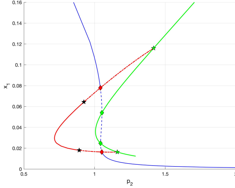
Figure 16: Families of equilibria (blue), saddle-node bifurcations of equilibria (green), and Hopf bifurcations of equilibria (red) for the vector field in Section 7.1. The Hopf bifurcation curve terminates at each end on the saddle-node bifurcation curve at a Bogdanov-Takens points (green star) and consists of both subcritical (dash-dotted) and supercritical (solid) bifurcations, separated by generalized Hopf bifurcations (black stars). While the location of the latter is accurate to within tolerance, the change in the sign of the Lyapunov coefficient is not detected until beyond this point, as evidenced by the crossing of the top-most generalized Hopf bifurcation by the dash-dotted curve.
