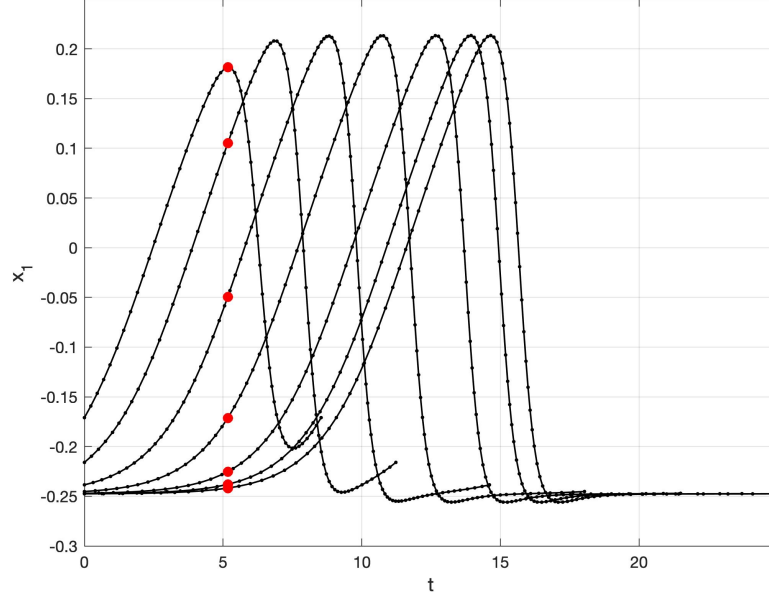
Figure 19: Time histories for labeled periodic orbits found during continuation using the code in Sect. 7.4 with points at t = 5.17 highlighted using red disks.
