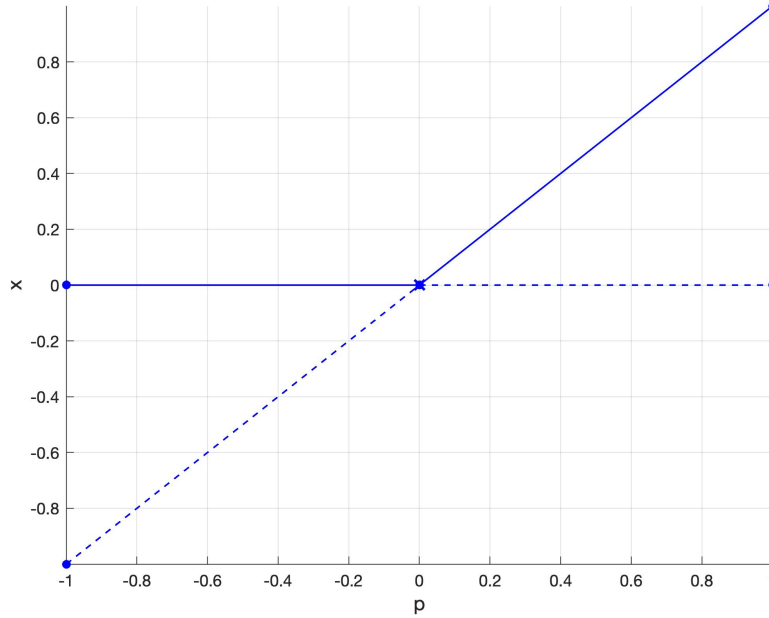
Figure 2: Bifurcation diagram showing branches of asymptotically stable (solid) and unstable (dashed) equilibria for the vector field in Section 3.2. The blue cross marks a branch point while the small blue disks mark the end points of each computation.
