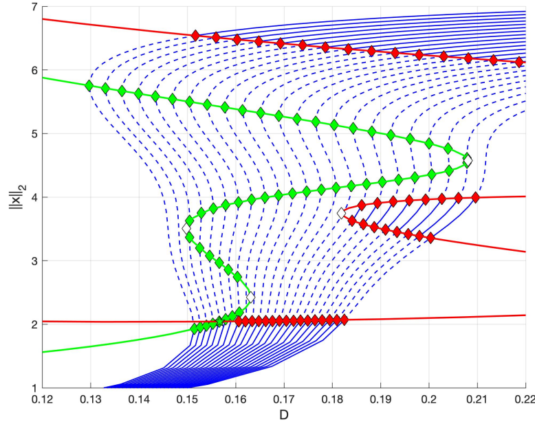
Figure 6: Bifurcation diagram showing branches of asymptotically stable (blue solid) and unstable (blue dashed) equilibria, saddle-node bifurcations (solid green), and Hopf bifurcations/neutral saddles (red solid) for the vector field in Section 3.5. The green and red diamonds mark saddle-node and Hopf bifurcations, the white diamonds mark fold points, and the green star at the intersection between the curves of saddle-node bifurcations and Hopf bifurcations/neutral saddles marks a Bogdanov-Takens point.
