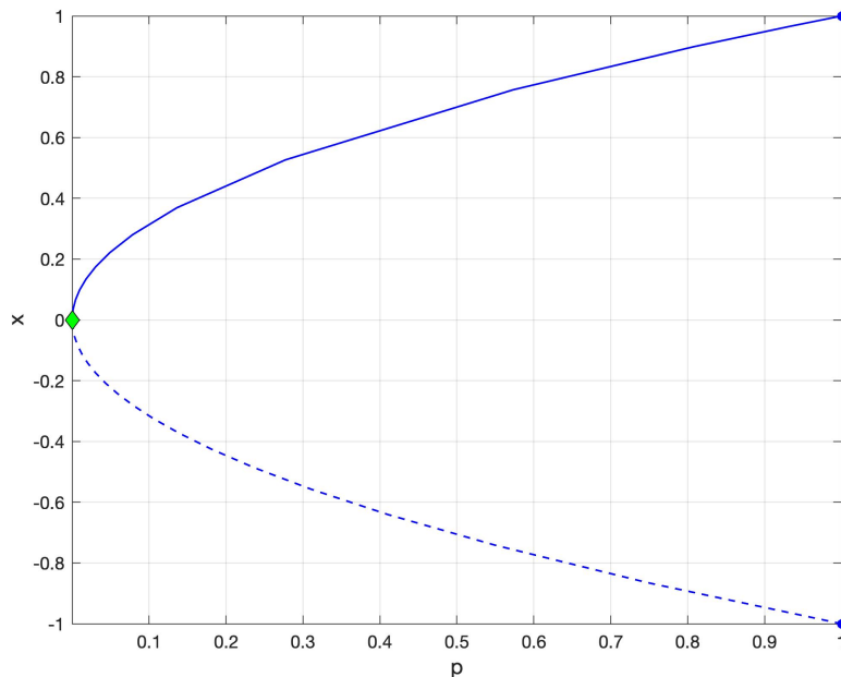
Figure 1: Bifurcation diagram showing branches of asymptotically stable (solid) and unstable (dashed) equilibria for the vector field in Section 3.1. The green diamond marks a saddle-node bifurcation while the small blue disks mark the end points of the computation.
