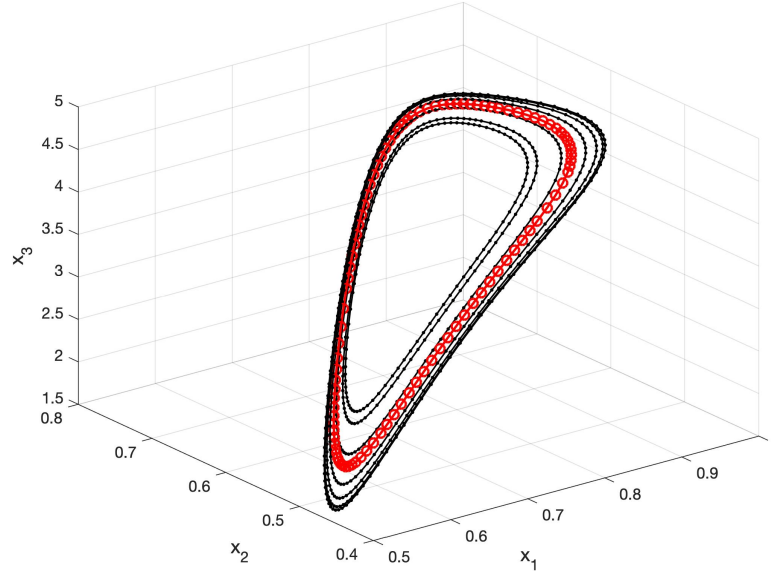
Figure 13: One-dimensional family of periodic orbits at saddle-node bifurcations for the vector field in Section 4.2. The orbit found at a fold point along this family is highlighted in solid red.
