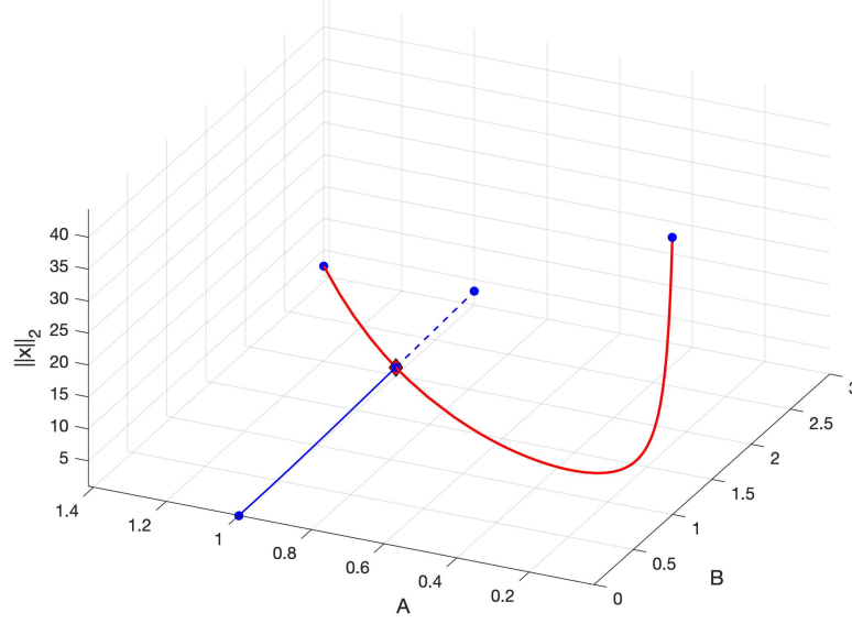
Figure 4: Bifurcation diagram showing branches of asymptotically stable (blue solid) and unstable (blue dashed) equilibria and Hopf bifurcations (solid red) for the vector field in Section 3.4. The red diamond marks a Hopf bifurcation, while the small blue disks mark the end points of each computation.
