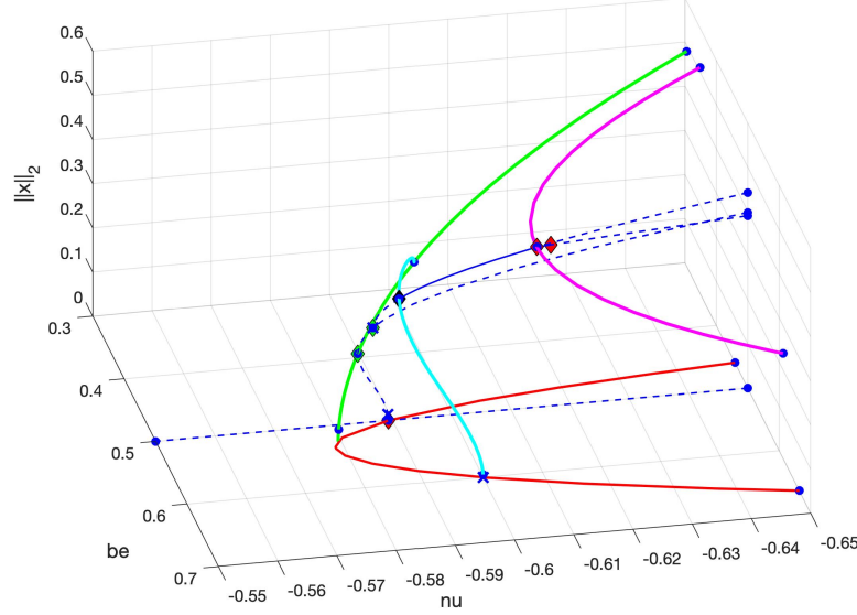
Figure 10: Bifurcation diagram showing branches of unstable (blue dashed) equilibria, Hopf bifurcations of equilibria (red solid) asymptotically stable (blue solid) and unstable (blue dashed) periodic orbits, saddle-node bifurcations of periodic orbits (green solid), period-doubling bifurcations (magenta solid), and torus bifurcations (cyan solid) for the vector field in Section 4.3. The green, blue, and red diamonds along curves of periodic orbits mark saddle-node, torus, and period-doubling bifurcations.
