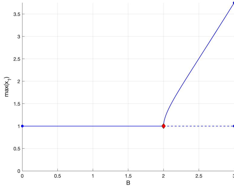
Figure 14: One-dimensional family of equilibria and one-dimensional family of asymptotically stable periodic orbits emanating from a supercritical Hopf bifurcation (red diamond) for the vector field in Section 6.3.
