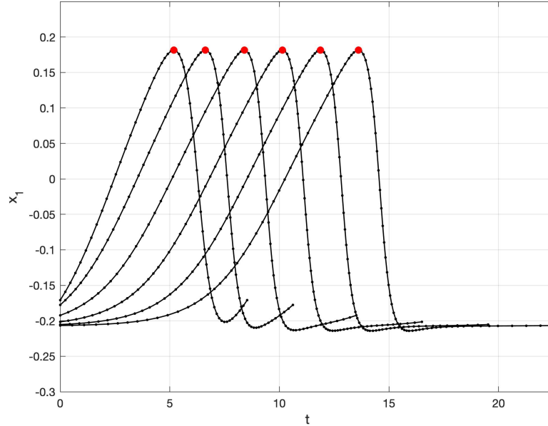
Figure 21: Time histories for labeled periodic orbits found during continuation using the code in Sect. 7.4 with a family of local maxima highlighted using red disks.
