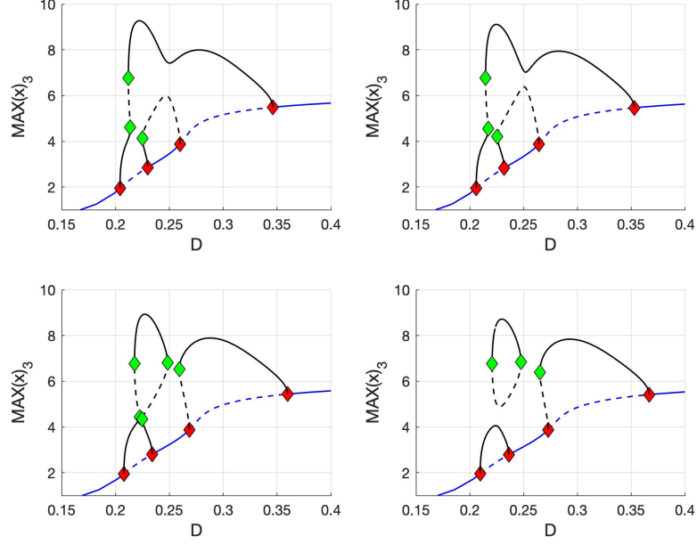
Figure 9: Bifurcation diagram showing branches of asymptotically stable (blue solid) and unstable (blue dashed) equilibria, as well as asymptotically stable (black solid) and unstable (black dashed) periodic orbits for the vector field in Section 4.2. The green and red diamonds mark saddle-node and Hopf bifurcations. The diagram differs from that in Fig. 8 by the inclusion of the isolated curve of periodic orbits in the bottom right panel.
