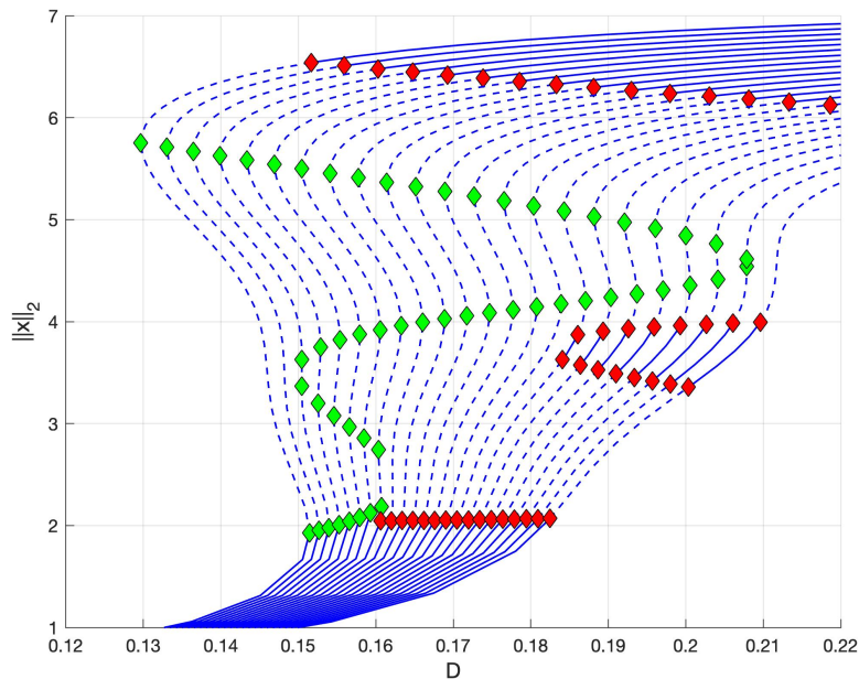
Figure 5: Bifurcation diagram showing branches of asymptotically stable (blue solid) and unstable (blue dashed) equilibria for the vector field in Section 3.5. The green and red diamonds mark saddle-node and Hopf bifurcations, respectively.
