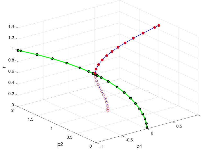
Figure 17: Comparison between theoretical predictions (red and black balls) and the results of continuation along families of periodic orbits (blue solid) and saddle-node bifurcations of periodic orbits (green solid) associated with the Hopf normal form in Sec. 4.1. The vertical coordinate r represents the projection onto the Fourier coefficient associated with \cos t .
