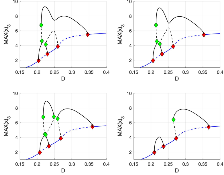
Figure 8: Bifurcation diagram showing branches of asymptotically stable (blue solid) and unstable (blue dashed) equilibria, as well as asymptotically stable (black solid) and unstable (black dashed) periodic orbits for the vector field in Section 4.2. The green and red diamonds mark saddle-node and Hopf bifurcations.
