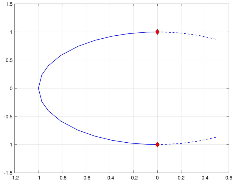
Figure 12: Bifurcation diagram showing the progression in the complex plane of the eigenvalues of the Jacobian of the vector field with respect to the state versus the parameter B for the vector field in Section 3.4. The red diamonds mark the Hopf bifurcation as the pair of eigenvalues crosses the imaginary axis.
