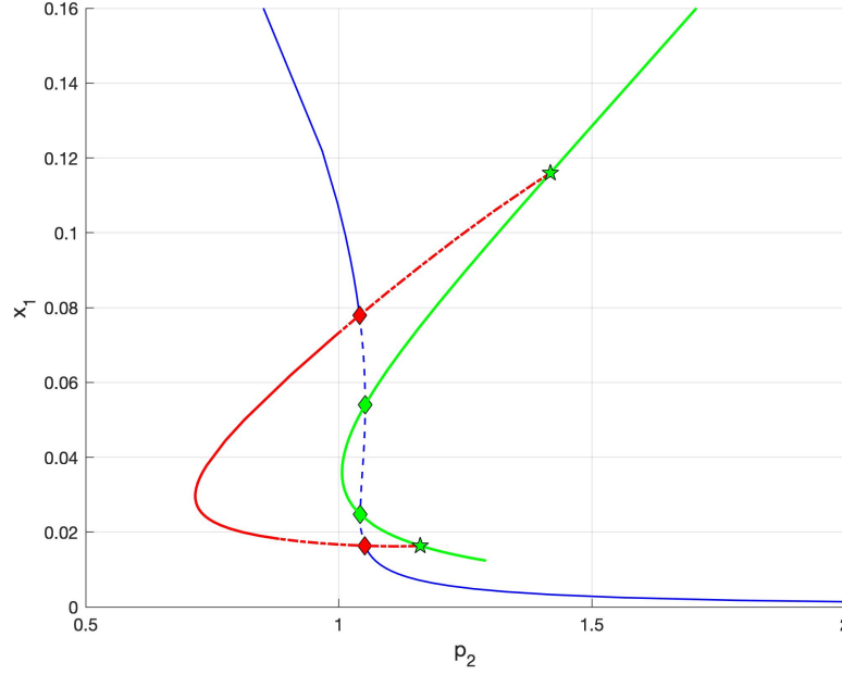
Figure 15: Families of equilibria (blue), saddle-node bifurcations of equilibria (green), and Hopf bifurcations of equilibria (red) for the vector field in Section 7.1. The Hopf bifurcation curve terminates at each end on the saddle-node bifurcation curve at a Bogdanov-Takens points (green star) and consists of both subcritical (dash-dotted) and supercritical (solid) bifurcations.
