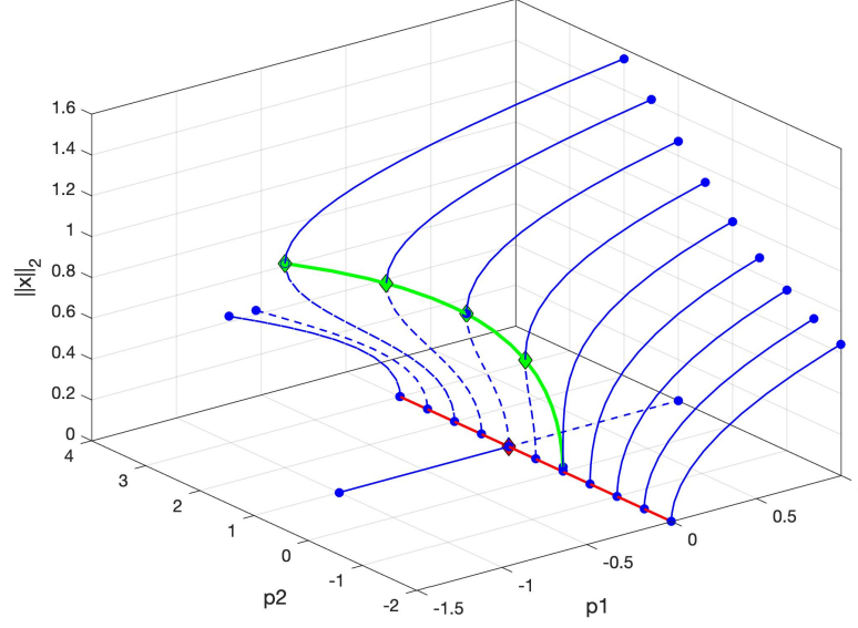
Figure 7: Bifurcation diagram showing branches of asymptotically stable (blue solid) and unstable (blue dashed) equilibria and periodic orbits, saddle-node bifurcations of periodic orbits (solid green), and Hopf bifurcations (red solid) for the vector field in Section 4.1. The green and red diamonds mark saddle-node and Hopf bifurcations, and the blue disks mark the end points of each computation.
